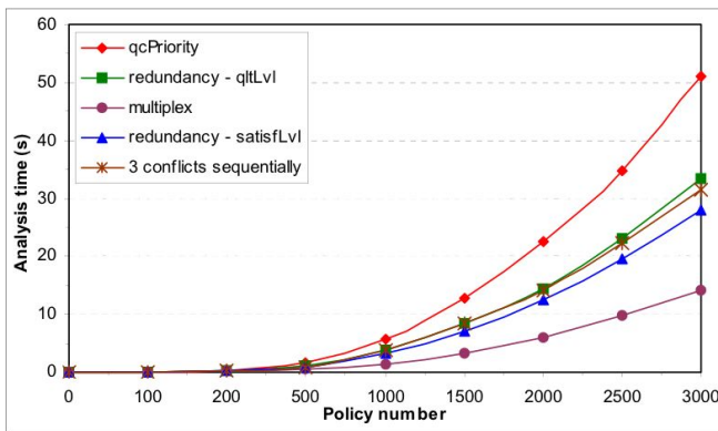
Fig. 9. Detection performance against number of policies for different conflict types.
