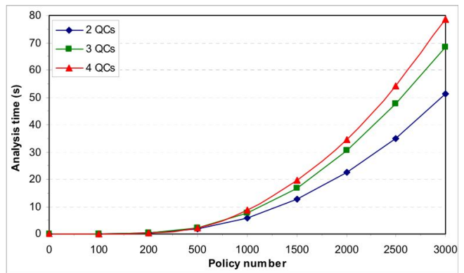
Fig. 8. Detection performance against number of policies with varying QCs.
