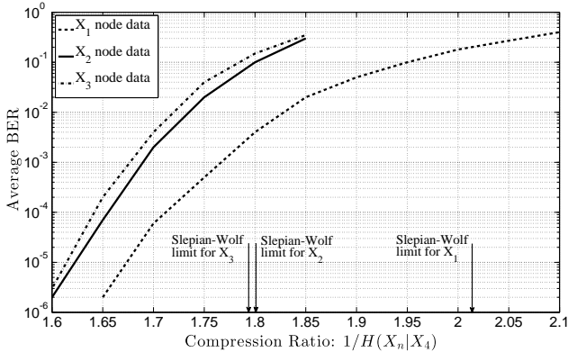
Figure 5: Average BER of the decoded information vs. the compression ratio.
