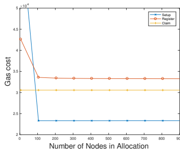
Fig. 4: Progression of gas costs for functions of the billboard contract using off-chain storage of nodes.
