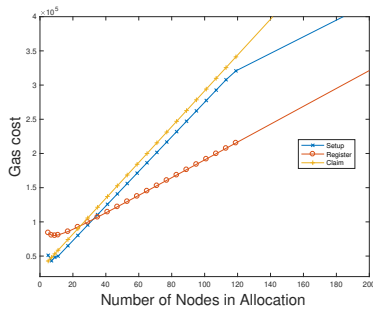
Fig. 3: Progression of gas costs for functions of the billboard contract using on-chain storage of nodes.
