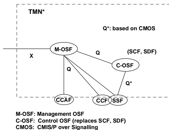
Fig. 4. Realising the IN through the Enhanced TMN (TMN*)
