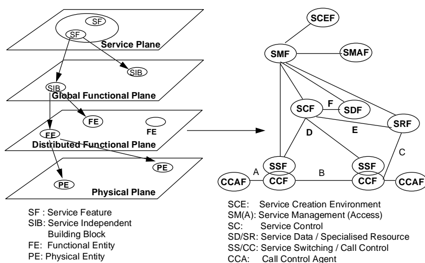
Fig. 2. The IN Layered and Functional Architecture
