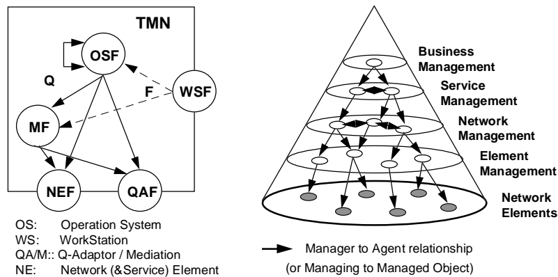
Fig. 3. The TMN Functional and Layered Architecture
