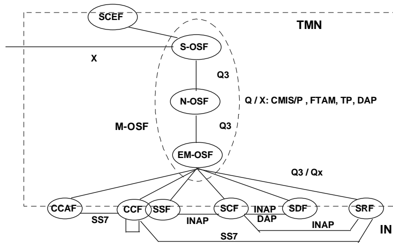
Fig. 1. Relationship between IN (control) and TMN (management)
