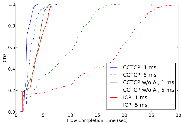
Fig. 5: Impact of link propagation delay ( T_{link} ) on FCT (caching policy ALL+LRU, \alpha = 0.8 , C = 0.04P )
