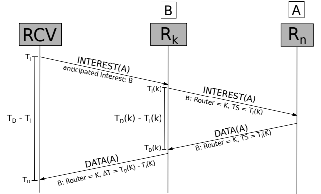
Fig. 1: RTT estimation and anticipated interests mechanism
